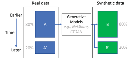
Figure 11: NetFlow traffic type prediction setup
