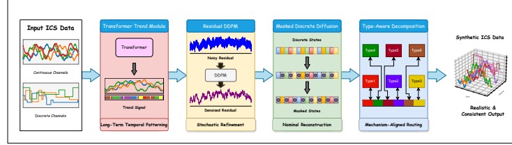
Fig. 1. Masked-DDPM: Unified Synthesis for ICS traffic
